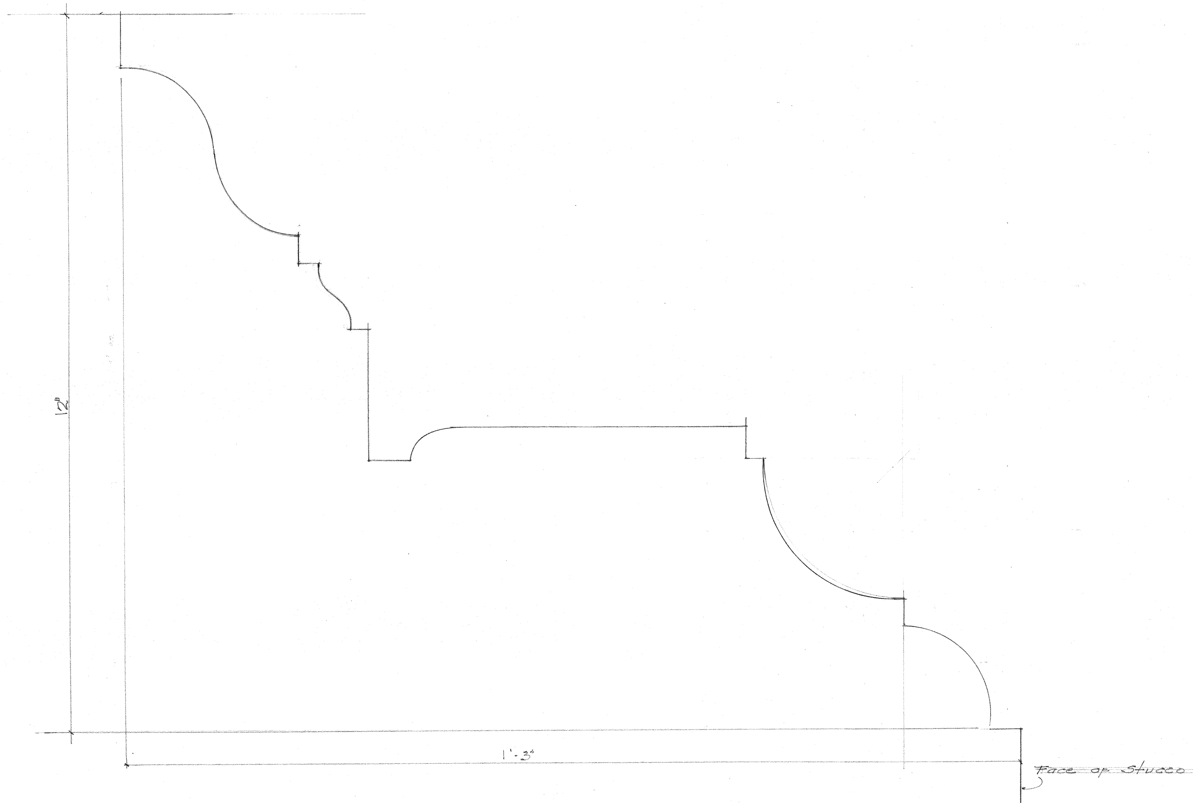
F.S. PROFILE FOR MAIN CORNICE & TOWER CORNICE
